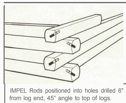
Diagram 3 Typical Butt and Pass Corner
